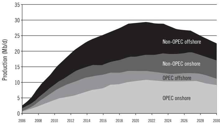
Figura 2: IEA production forecast for fields yet to be developed.
