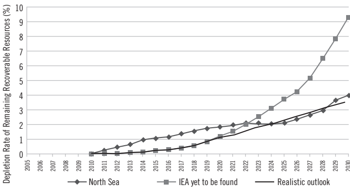
Figura 5: Depletion rates for the North Sea and fields yet to be found.
