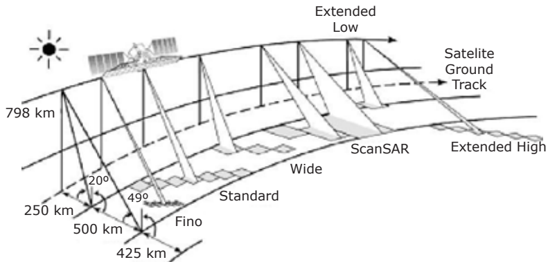
RADARSAT Beam Modes and Resolutions
