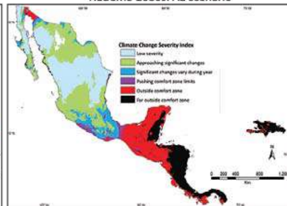
HadCM3 2080s: A2 scenario
