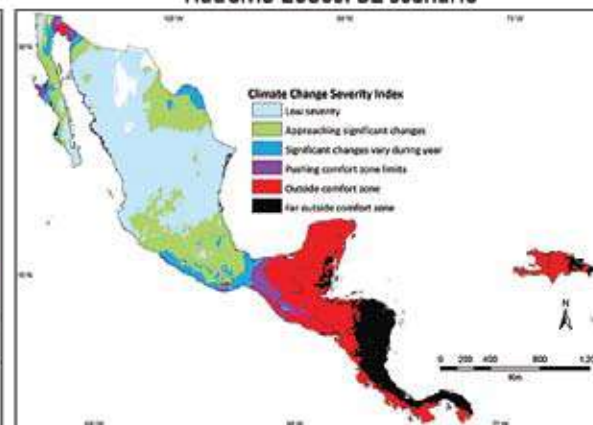
HadCM3 2080s: B2 scenario
