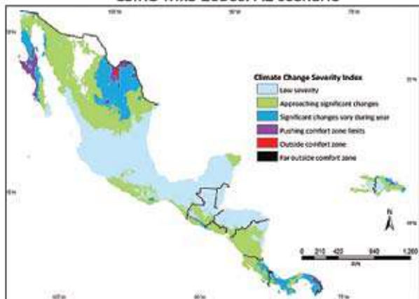
CSIRO Mk3 2050s: A2 scenario
