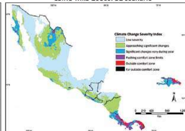
CSIRO Mk3 2080s: B2 scenario
