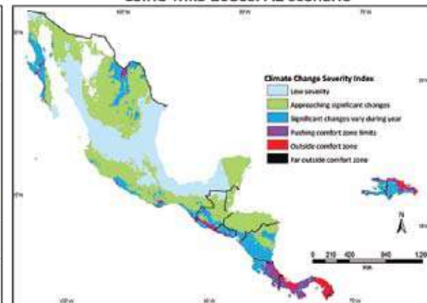
CSIRO Mk3 2080s: A2 scenario
