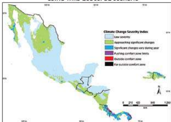
CSIRO Mk3 2050s: B2 scenario
