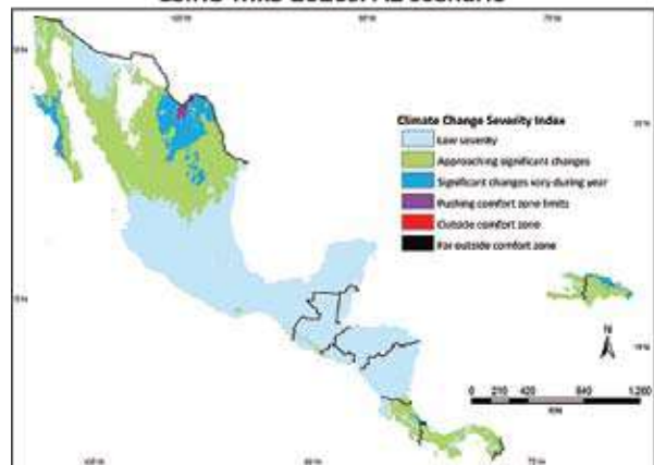
CSIRO Mk3 2020s: A2 scenario
