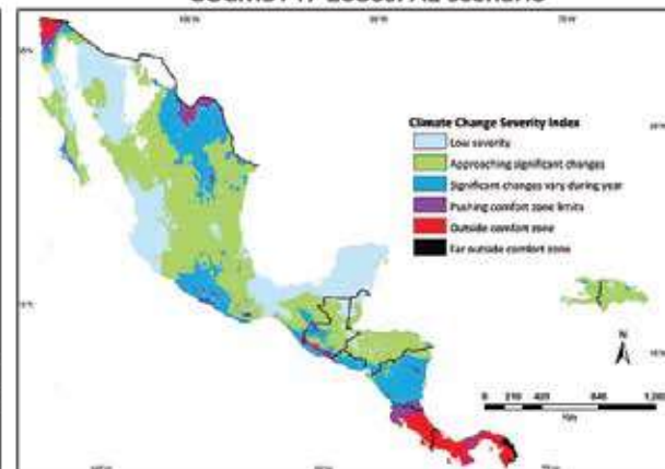
CGCM3T47 2080s: A2 scenario
