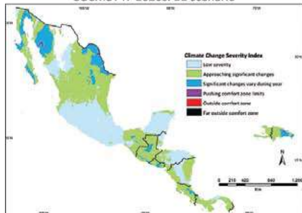
CGCM3T47 2020s: B2 scenario
