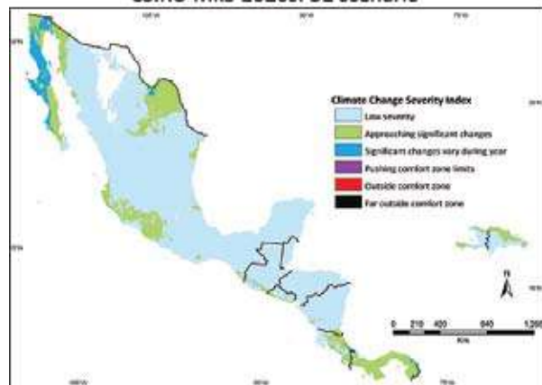
CSIRO Mk3 2020s: B2 scenario
