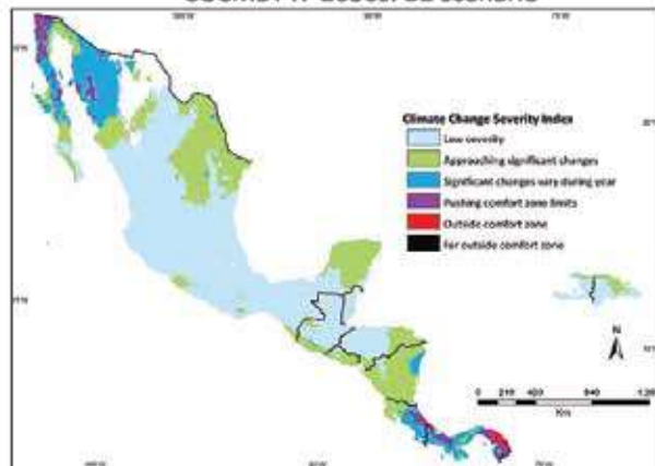
CGCM3T47 2050s: B2 scenario
